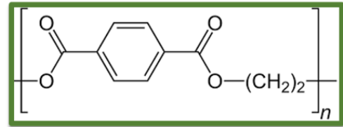
Polyethylene terephthalate
